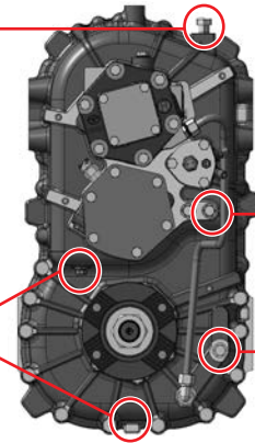
4. 브리더(Breather)
